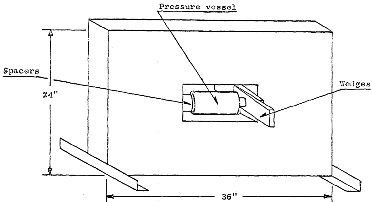
Clamping device with pressure vessel inserted
